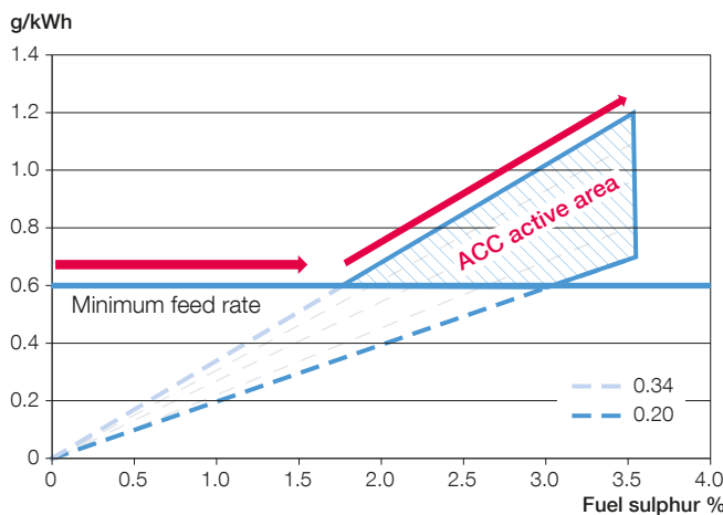
Fig. 1b: BN 70 ACC range Mk 7 and older
