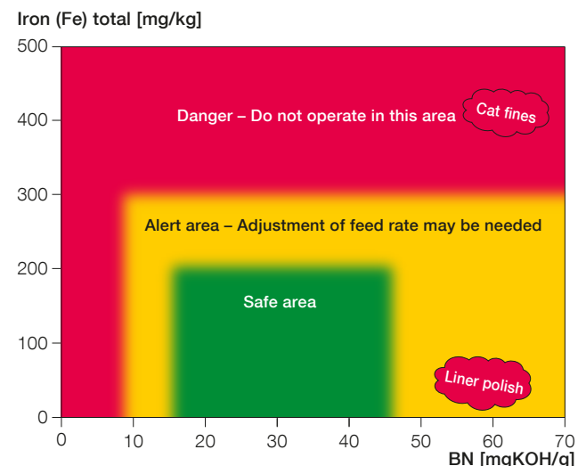
Fig. 2: Drain oil BN vs. iron (Fe)
